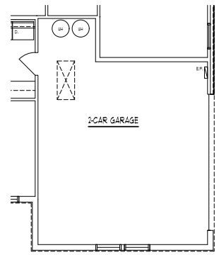
OPTIONAL SIDE ENTRY GARAGE FIRST FLOOR PLAN
