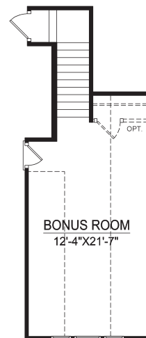
OPT. BONUS ROOM
